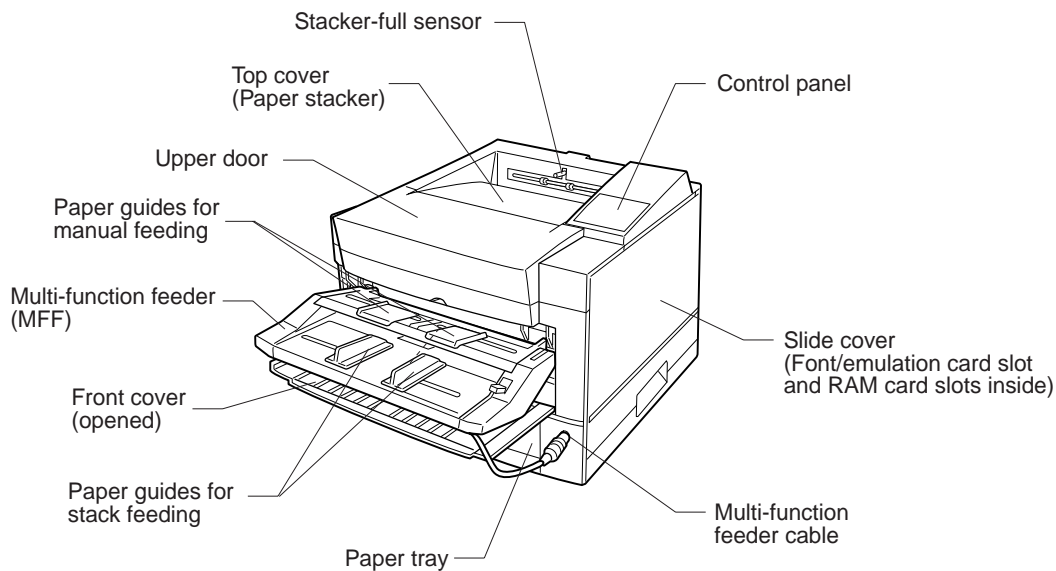
Figure 1-1 Front and right side view
